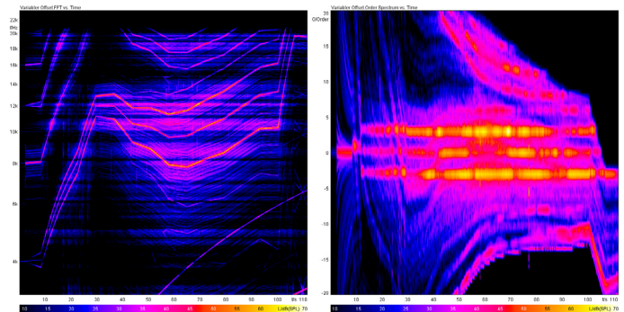
Variable Offset: FFT vs. Time, Order Spectrum vs. Time
