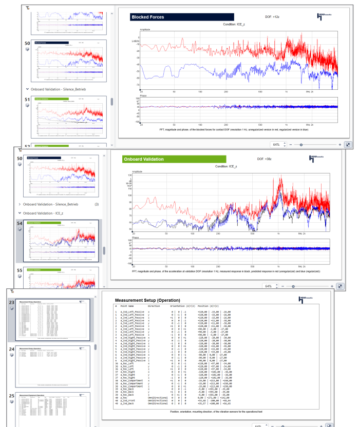
Automated generation of a test report in accordance with ISO 20270:2019
