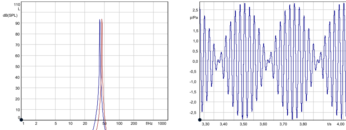
Figure 9: Frequency spectrum of two sinusoidal tones with small frequency difference (left); time signal of the resulting oscillation with beat (right)
