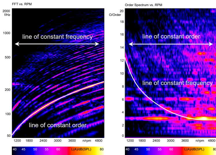
Figure 54: Comparison FFT and order analysis
