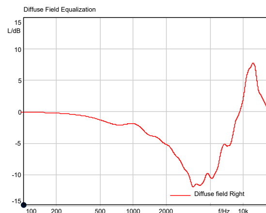
Figure 17: Diffuse field equalization for an artificial head measurement system HMS IV (right ear)
