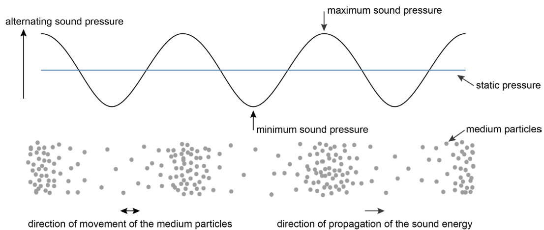
Figure 69: Generation of alternating sound pressure
