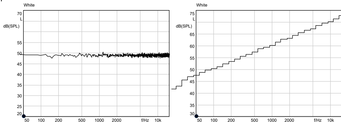
Figure 50: White noise; left: FFT analysis, right: 1/3-octave level analysis
