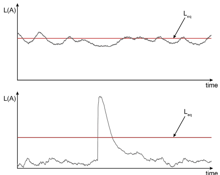
Figure 23: Equivalent continuous sound levels of a constant sound (top) and a transient sound (bottom)
