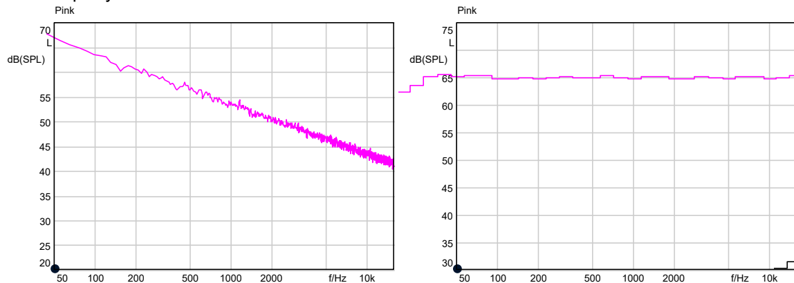
Figure 51: Pink noise; left: FFT analysis, right: 1/3-octave level analysis
