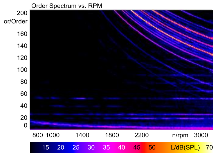
Figure 3: Order Spectrum vs. RPM of the signal analyzed in figure 1
